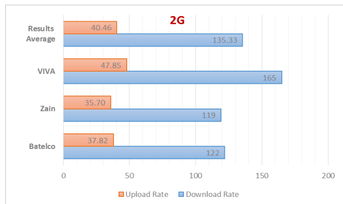
2G Download & Upload Transfer Rate (Kbps)
