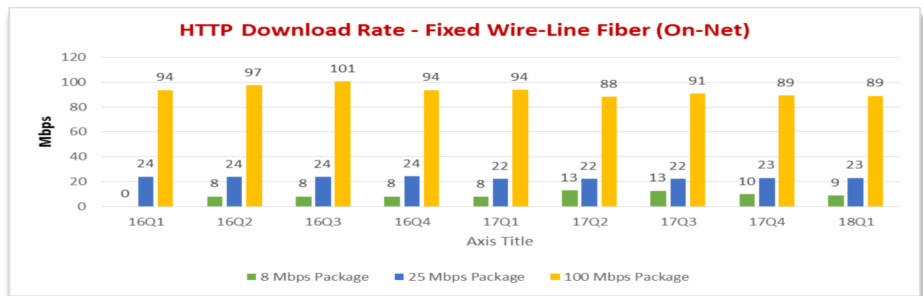
HTTP Download Rate - Fixed Wire-Line Fiber (On-Net) per Quarter Results Average
